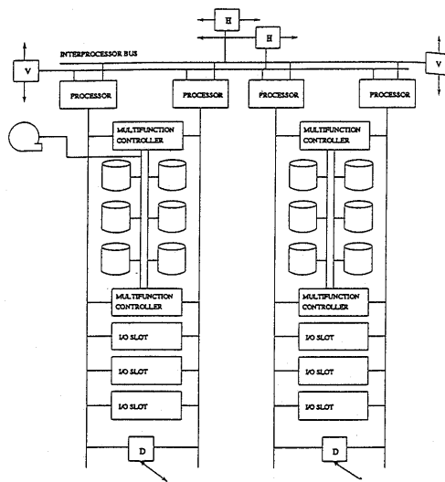
Tandem Himalaya K10000
