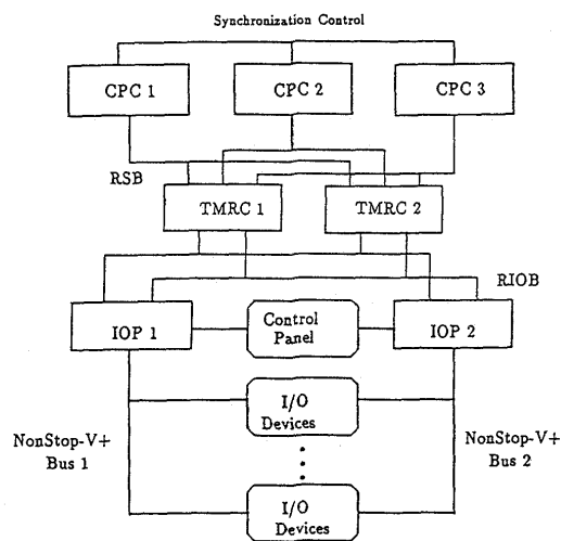
Tandem Integrity S2
