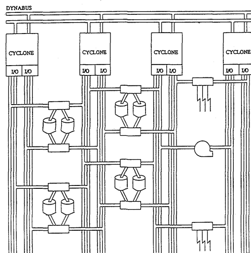
Tandem NonStop Cyclone
